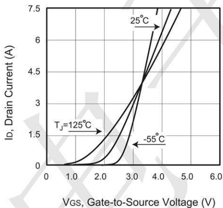
Figure 2. Transfer Characteristics
