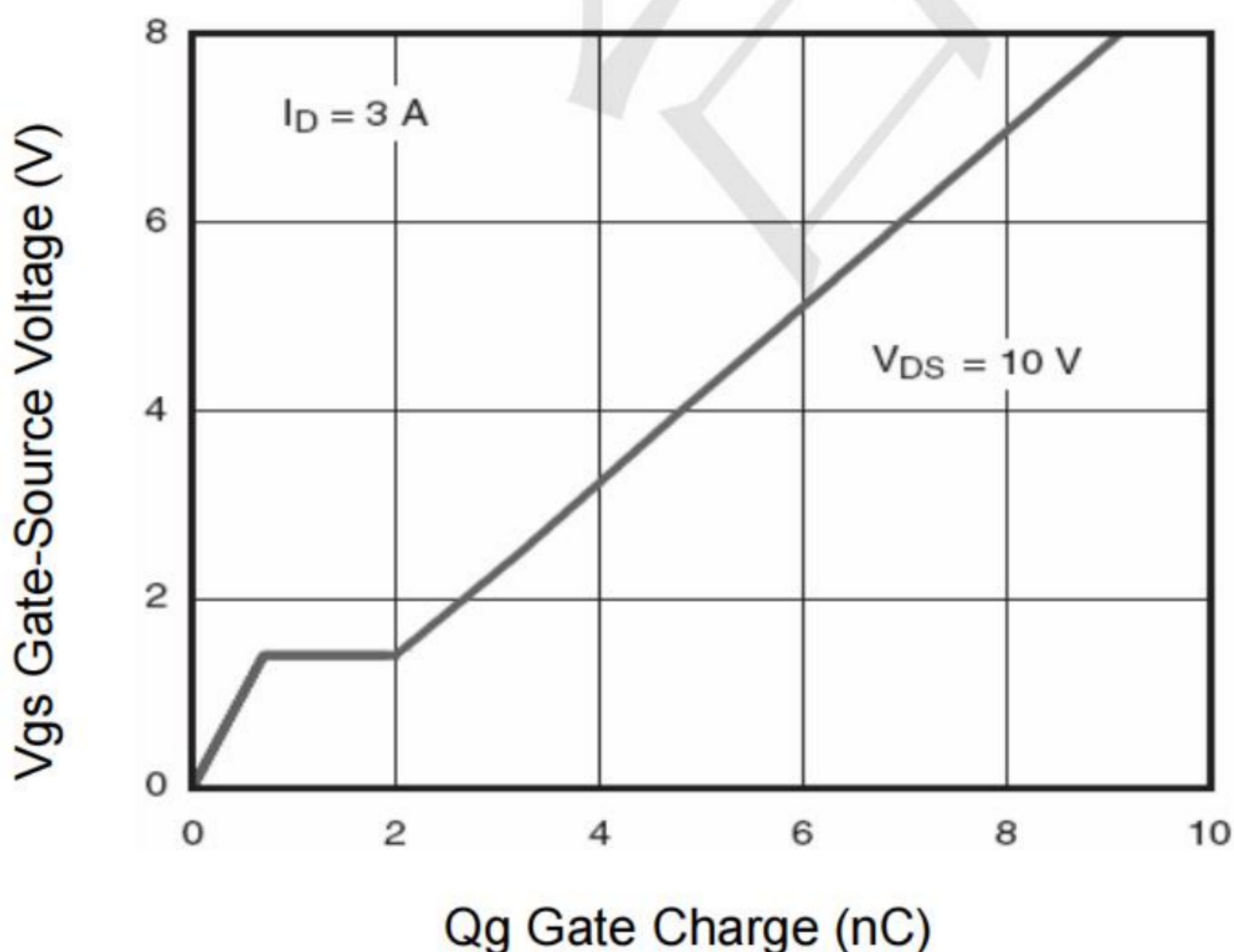
Figure 11 Gate Charge
