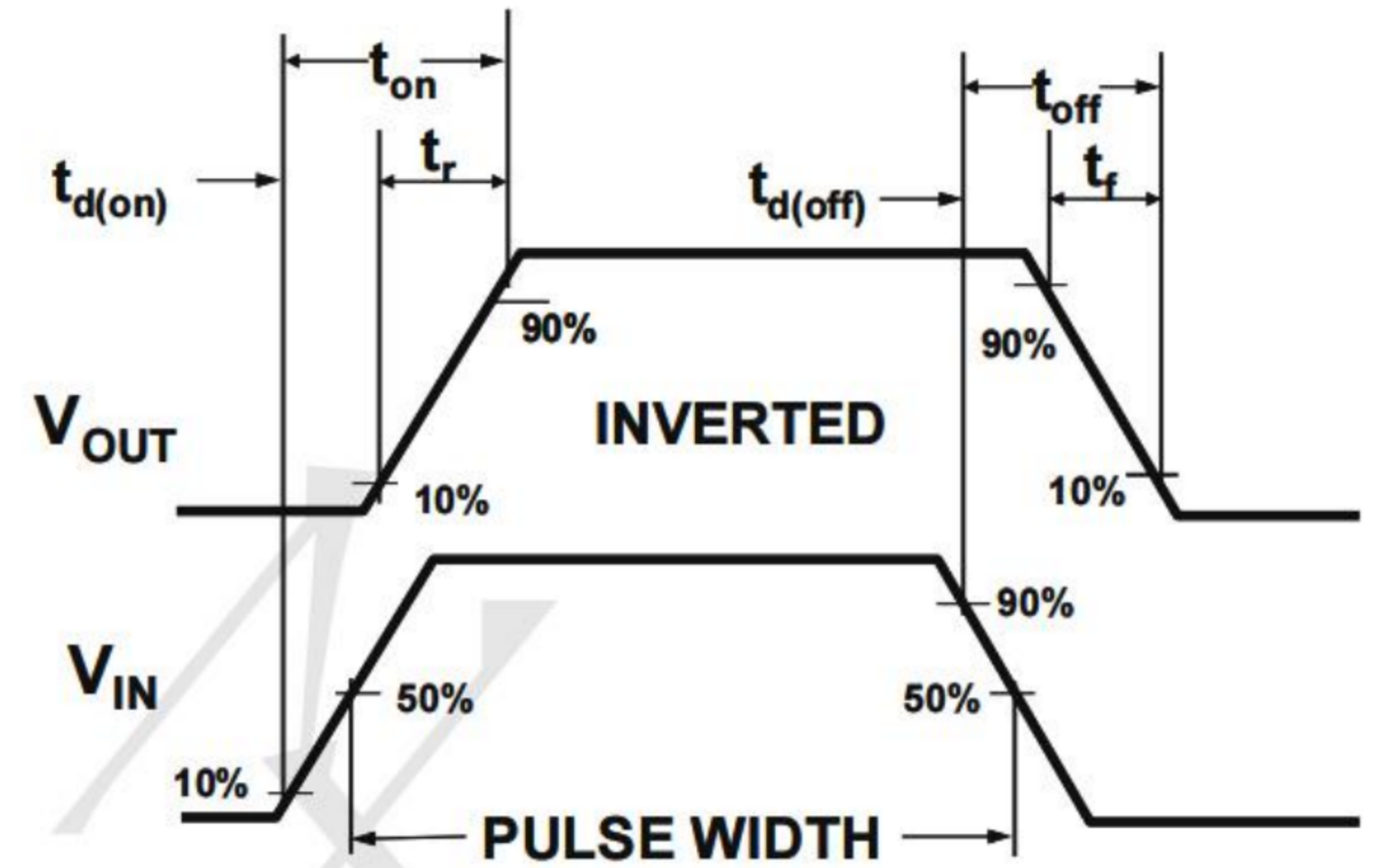
Figure 2: Switching Waveforms
