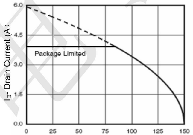
Figure 4 Drain Current
