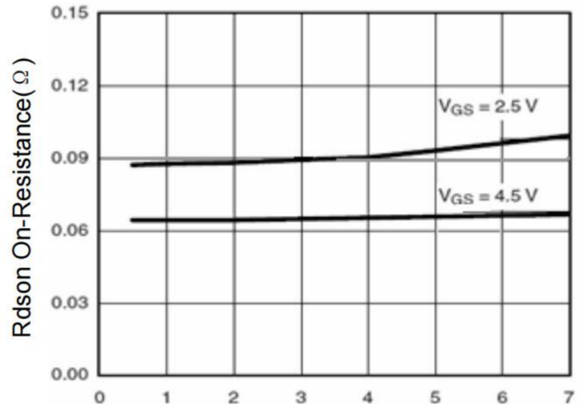
I_D - Drain Current (A) Figure 6 Drain-Source On-Resistance
