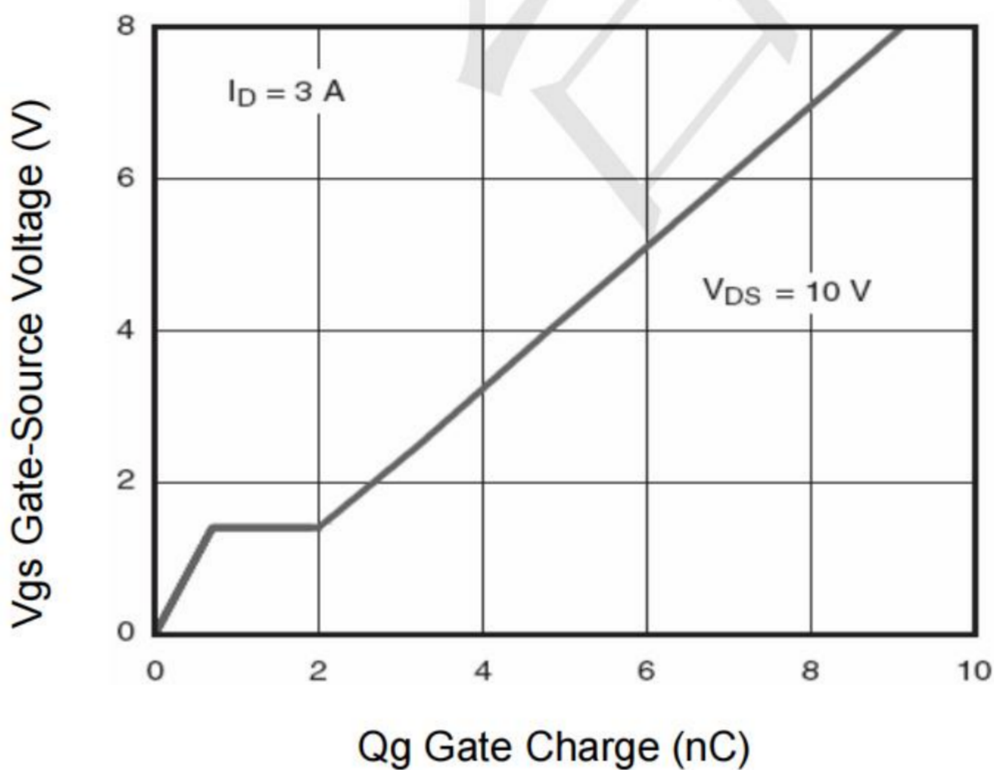
Figure 11 Gate Charge
