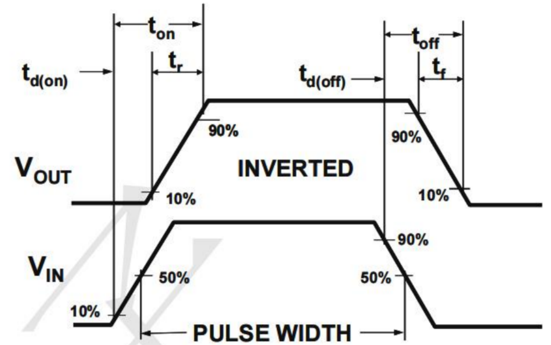
Figure 2: Switching Waveforms
