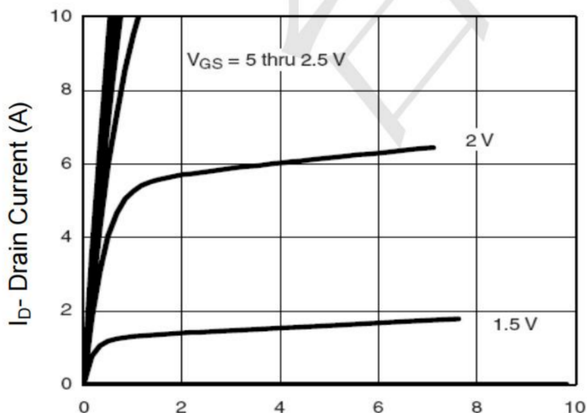
V_{DS} Drain-Source Voltage (V) Figure 5 Output Characteristics
