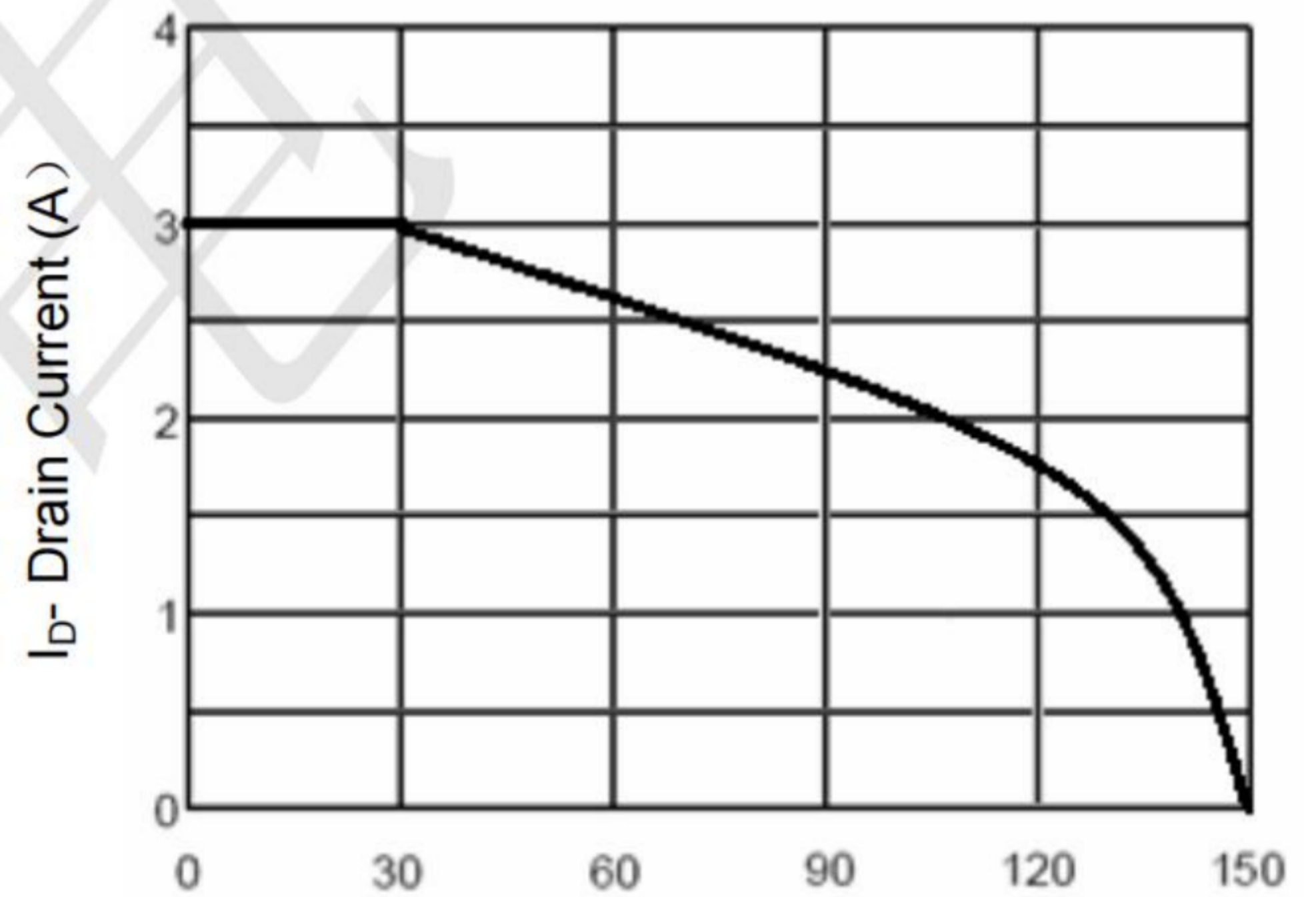
T_J -Junction Temperature (°C) Figure 4 Drain Current
