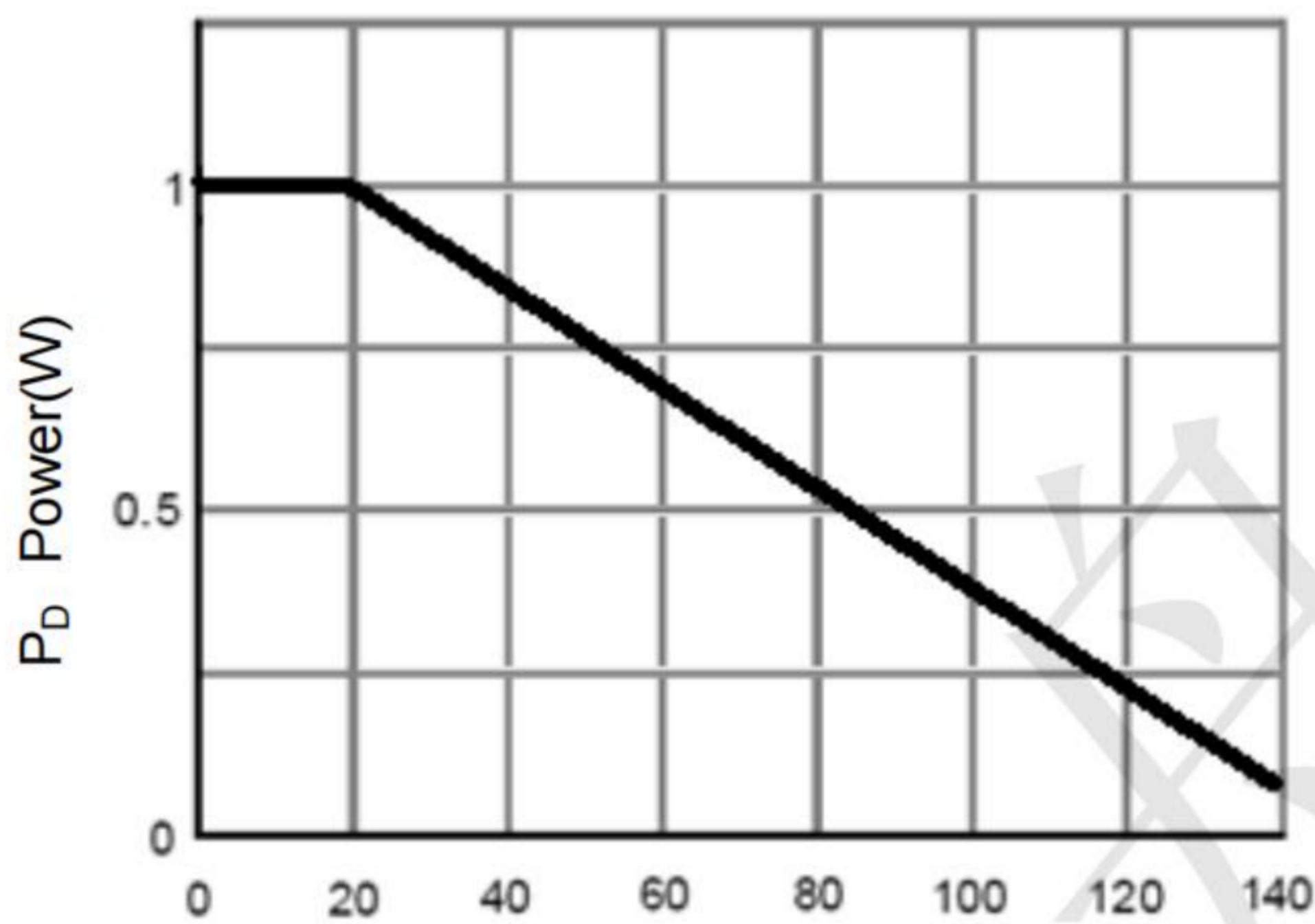
T_J -Junction Temperature ( ^{\circ}\text{C} ) Figure 3 Power Dissipation
