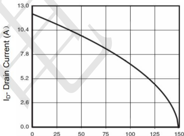
T J -Junction Temperature (°C) Figure 4 Drain Current
