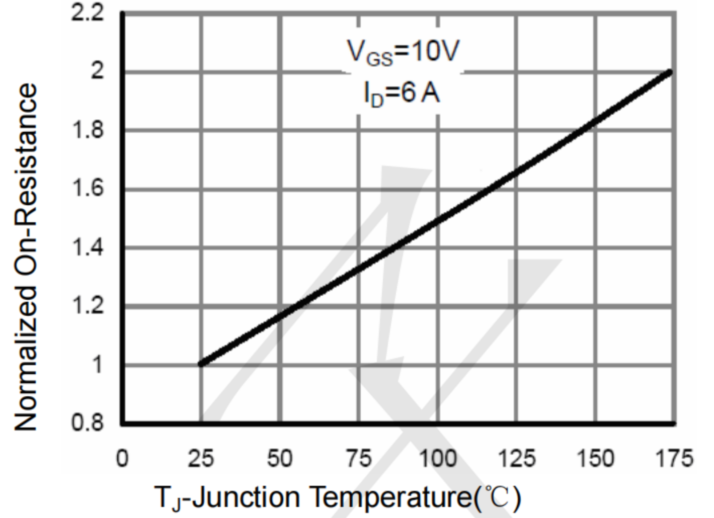
Figure 4 Rdson-Junction Temperature
