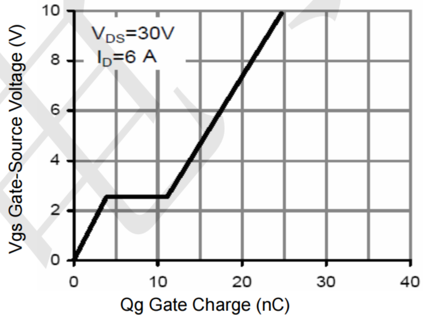
Figure 5 Gate Charge
