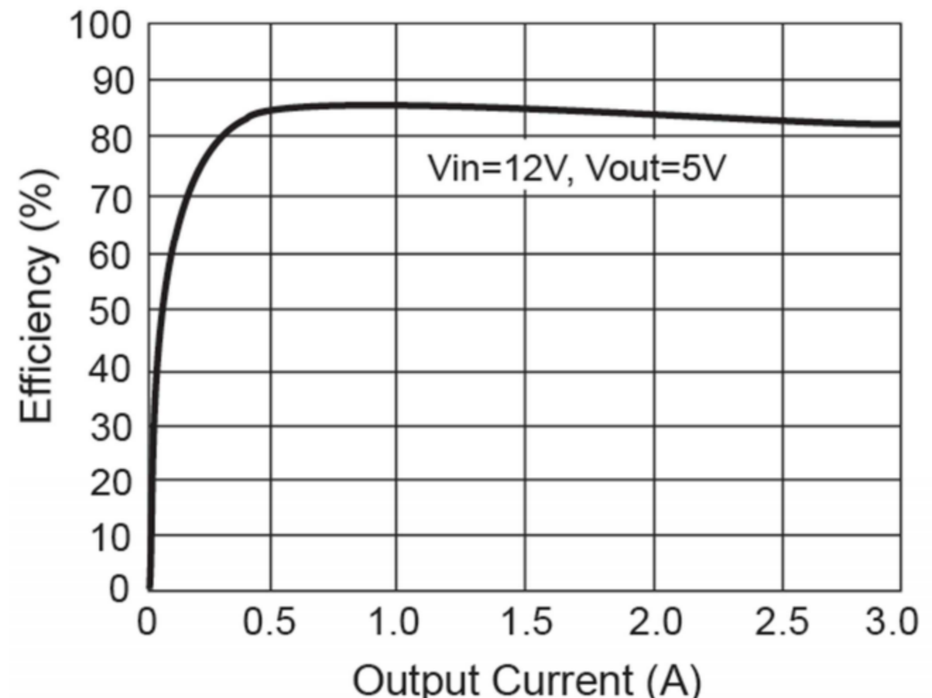
Figure 6. Efficiency
