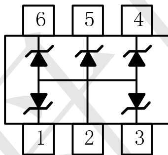
Pin Configuration
