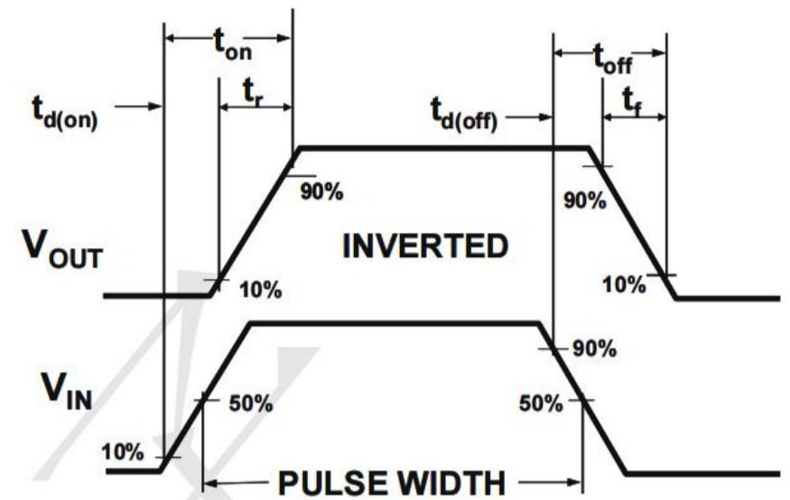
Figure 2: Switching Waveforms
