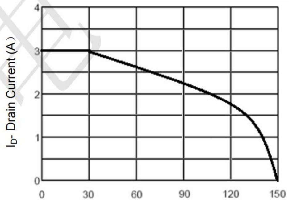
T_J -Junction Temperature (°C) Figure 4 Drain Current
