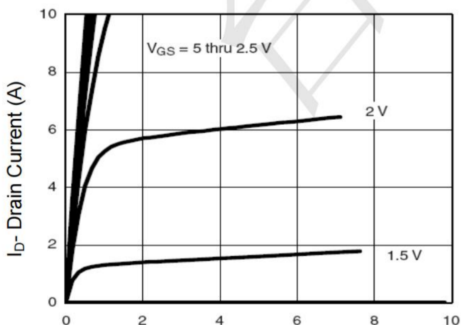
V_{DS} Drain-Source Voltage (V) Figure 5 Output Characteristics
