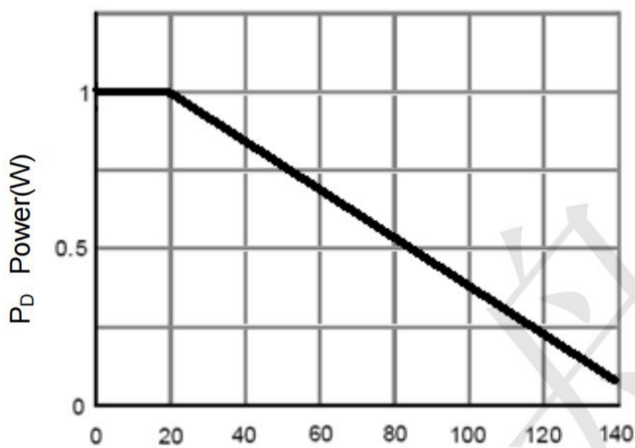
T_J -Junction Temperature (°C) Figure 3 Power Dissipation
