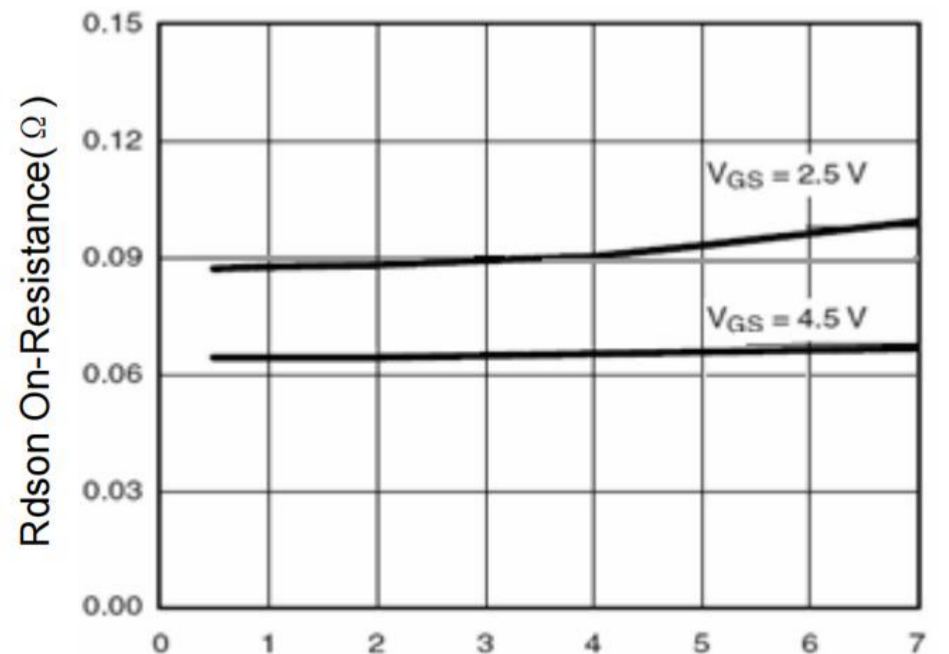
I_D - Drain Current (A) Figure 6 Drain-Source On-Resistance
