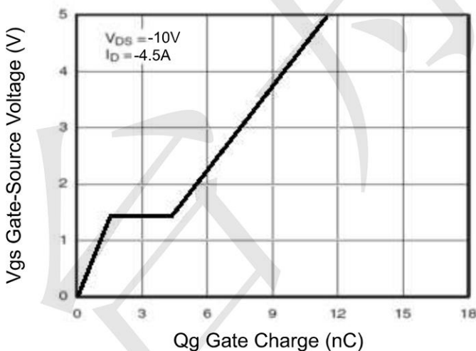
Figure 11 Gate Charge
