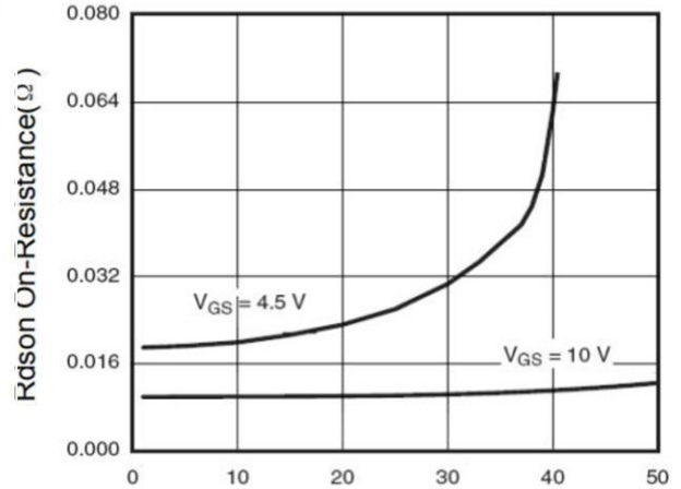
Figure 6 Drain-Source On-Resistance
