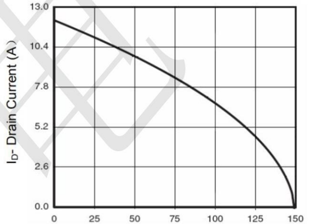
Figure 4 Drain Current
