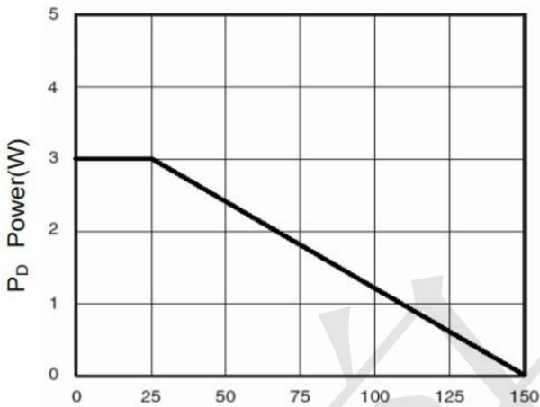
Figure 3 Power Dissipation
