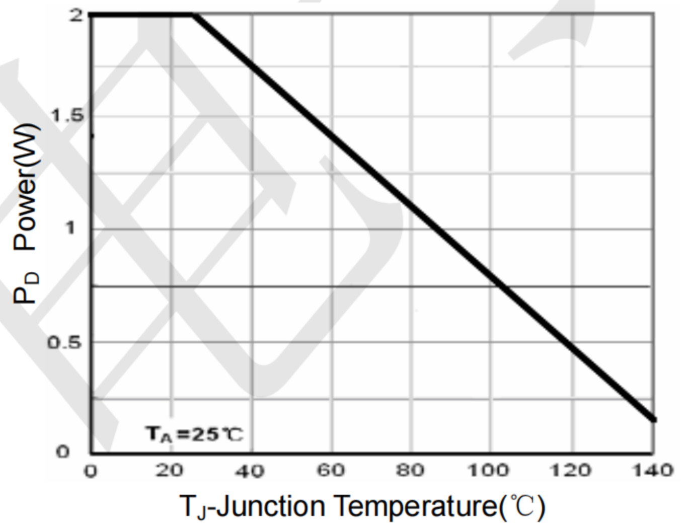
Figure 10 Power Dissipation
