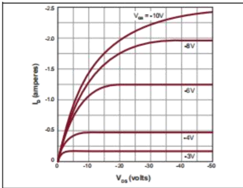
Output Characteristics.
