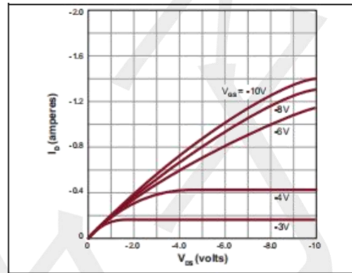
Saturation Characteristics.
