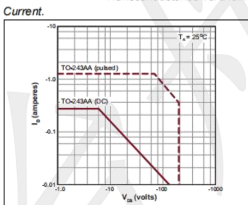
Maximum Rated Safe Operating Area.
