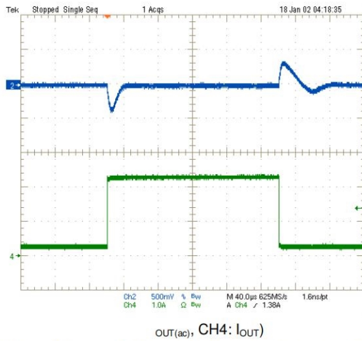
Fig. 13 Load Transient ( V_{IN}=12V , V_{OUT}=3.3V , I_O=0.25-2.25A )
