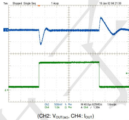
Fig. 14 Load Transient ( V_{IN}=12V , V_{OUT}=5V , I_O=0.25-2.25A )
