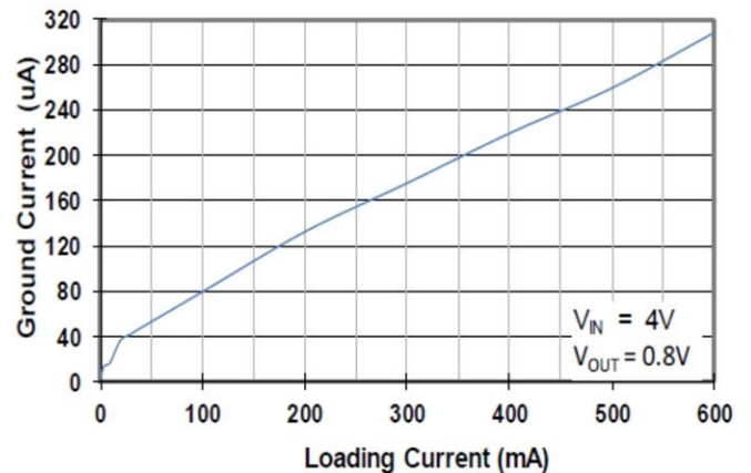
Fig. 10 Ground Current vs. Loading Current
