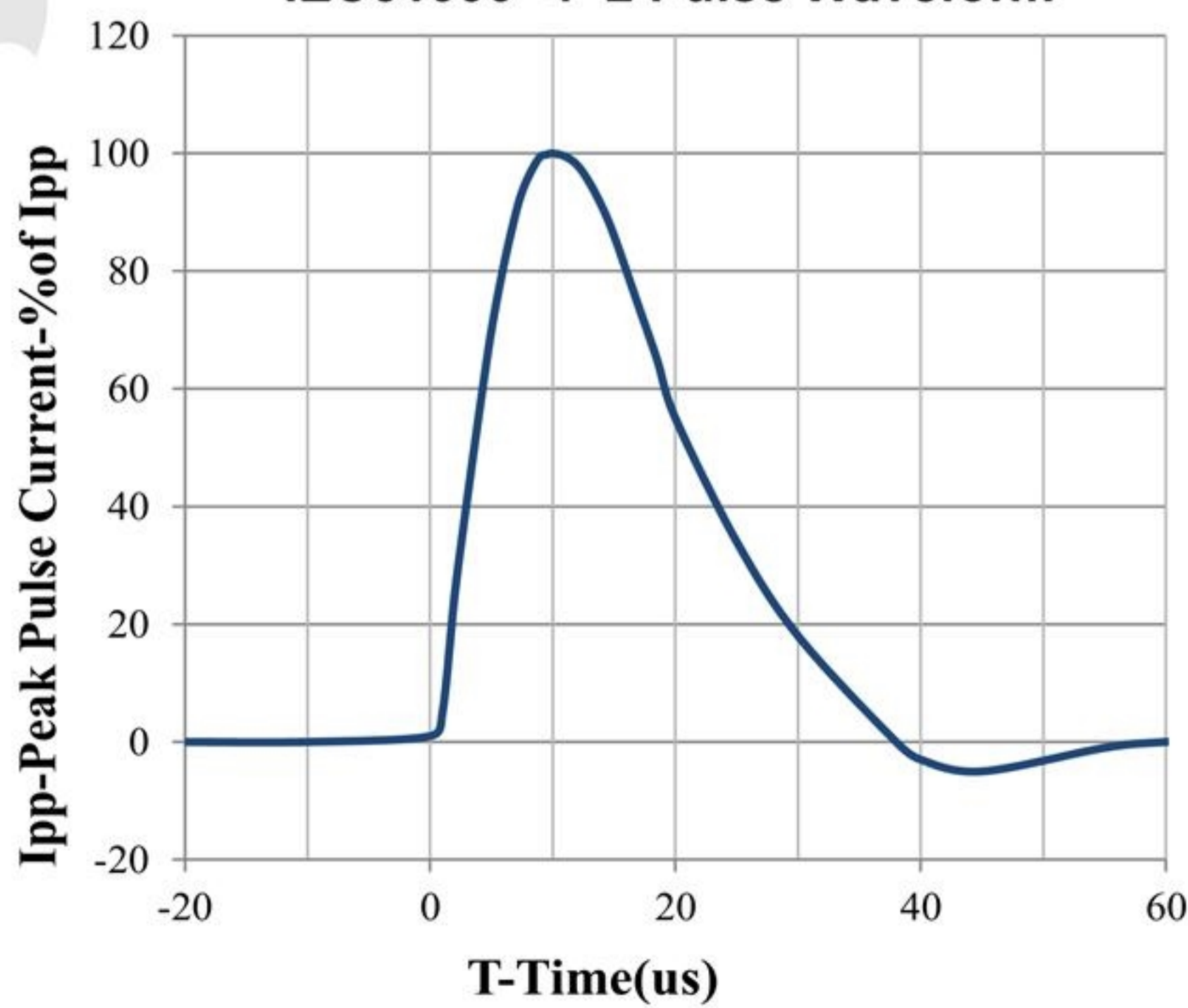
8 X 20us Pulse Waveform
