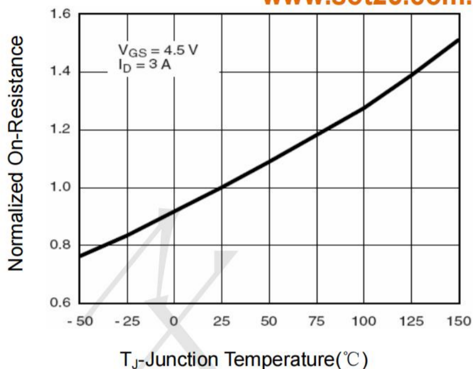
Figure 8 Drain-Source On-Resistance
