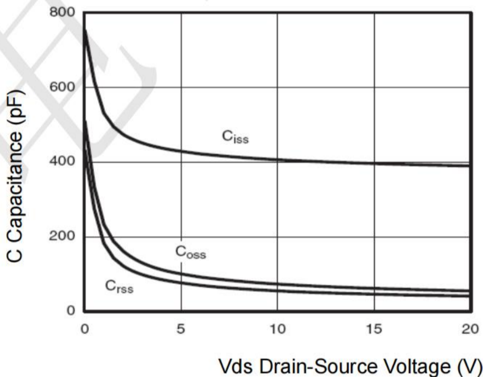
Figure 10 Capacitance vs Vds
