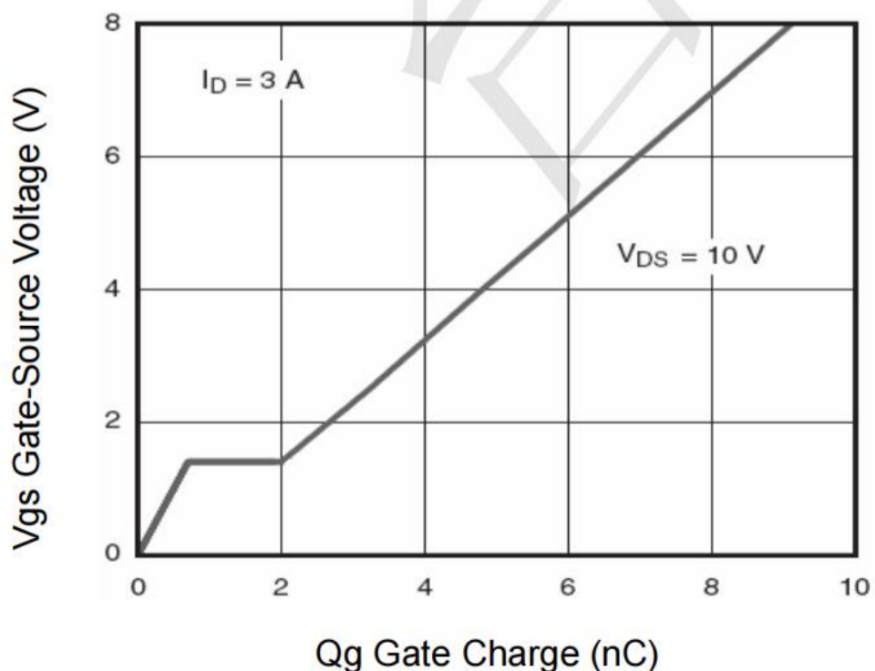
Figure 11 Gate Charge
