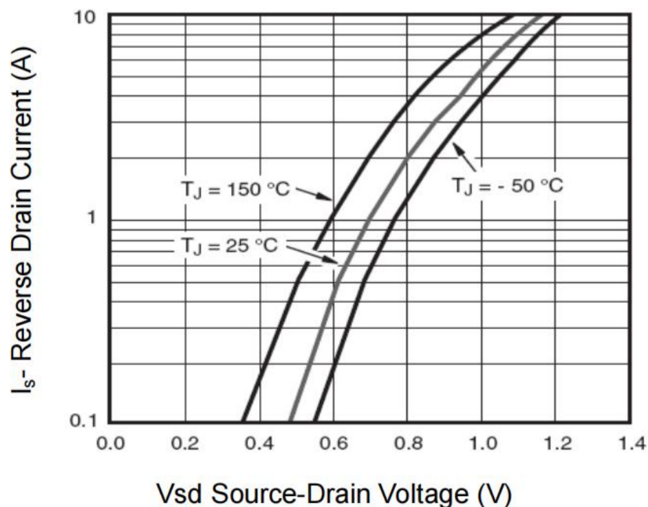
Figure 12 Source- Drain Diode Forward
