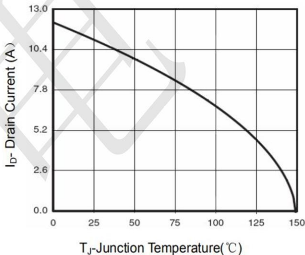
Figure 4 Drain Current
