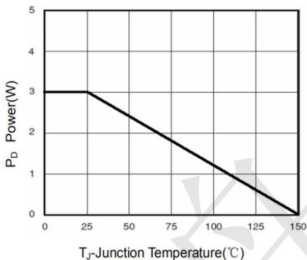
Figure 3 Power Dissipation
