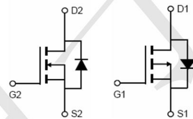
N-channel
