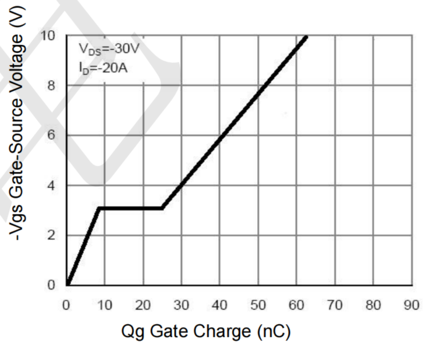
Figure 5 Gate Charge
