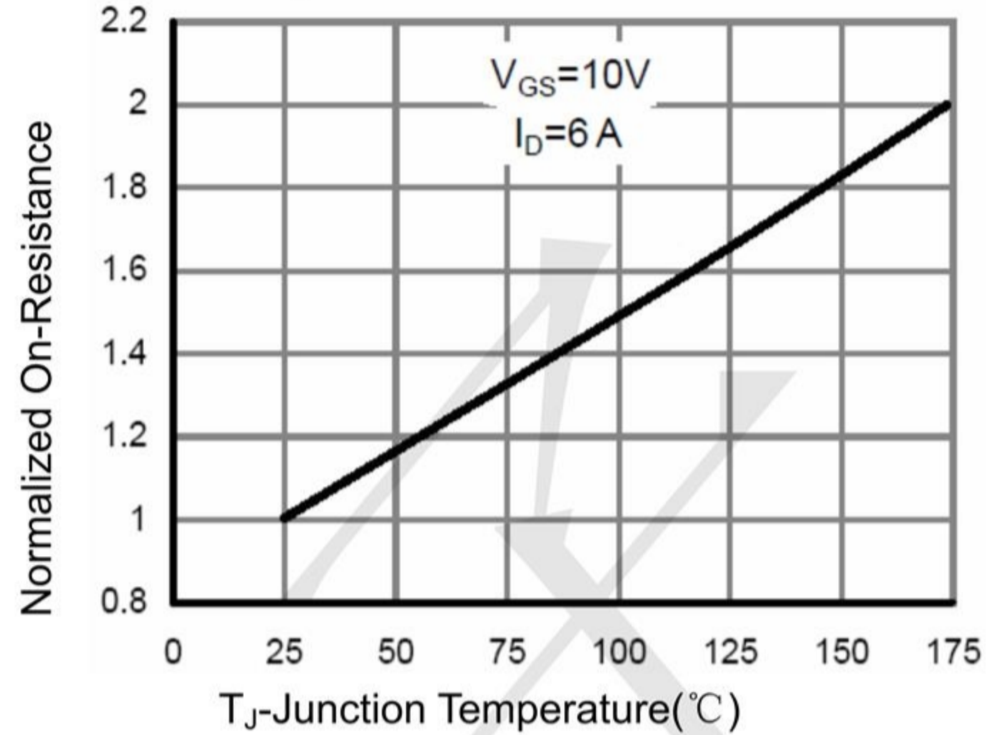
Figure 4 Rdson-Junction Temperature
