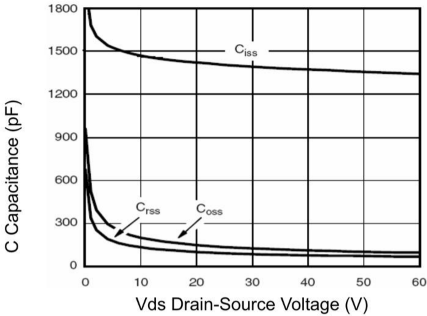
Figure 7 Capacitance vs Vds
