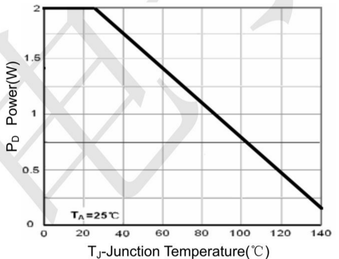
Figure 10 Power Dissipation
