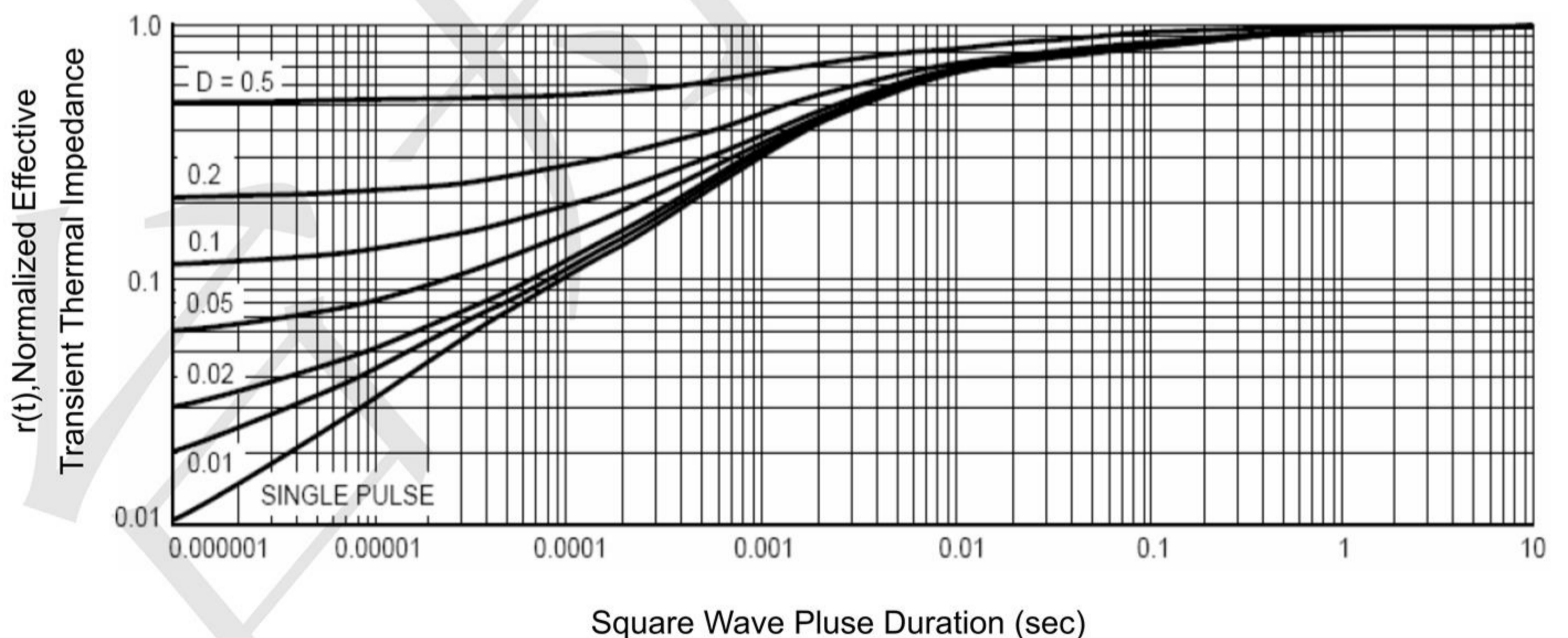
Figure 11 Normalized Maximum Transient Thermal Impedance
