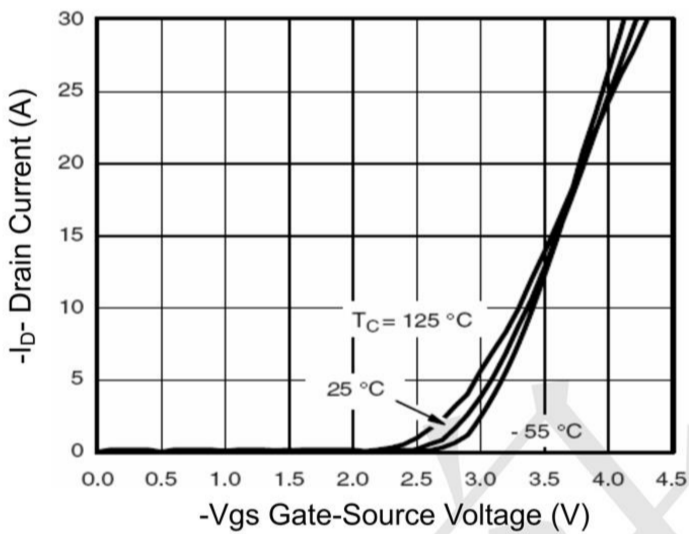
Figure 2 Transfer Characteristics
