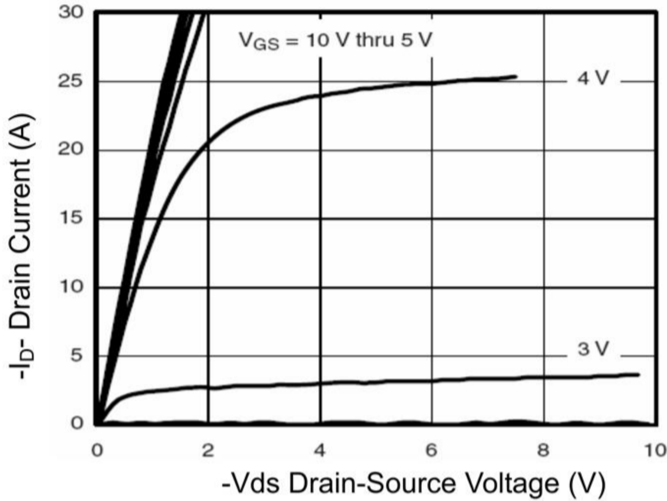
Figure 1 Output Characteristics
