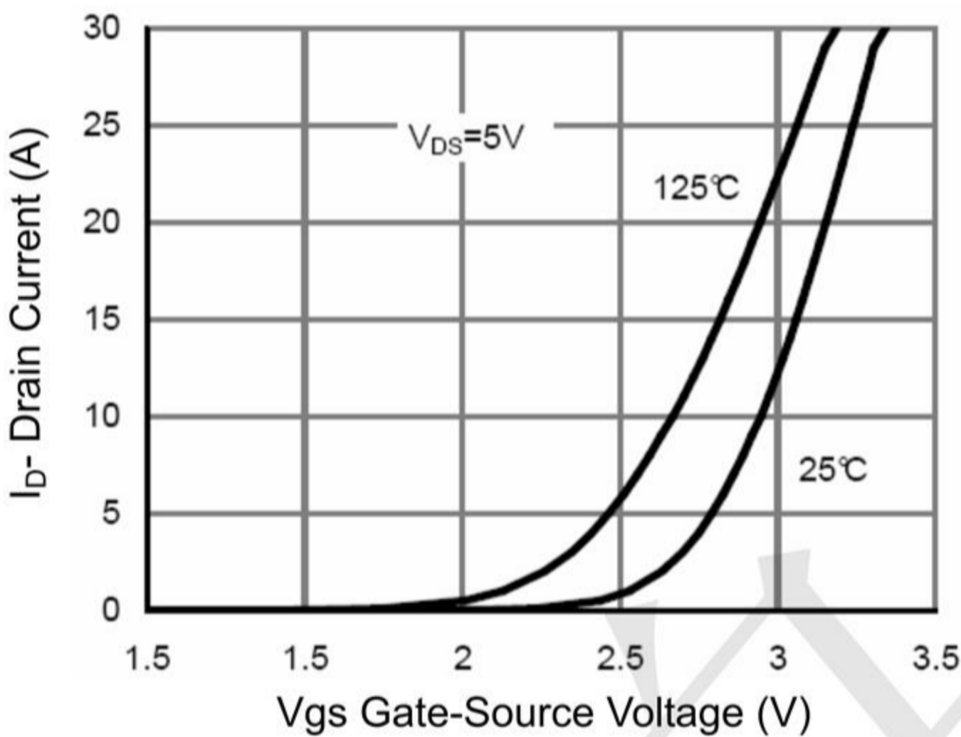
Figure 2 Transfer Characteristics
