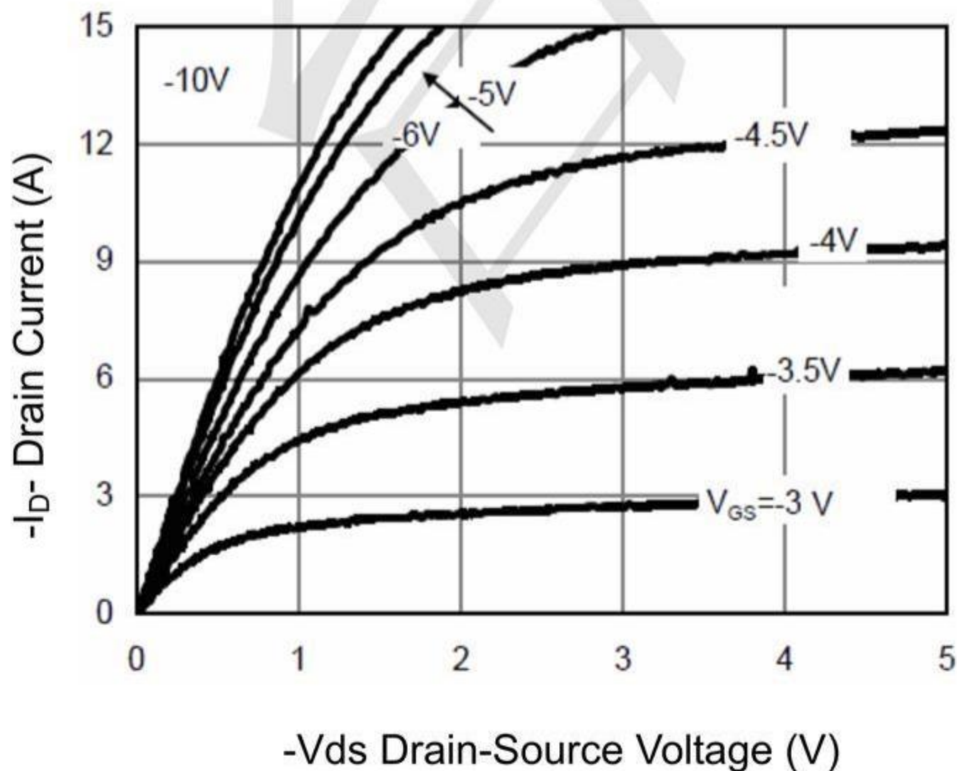
Figure 5 Output Characteristics
