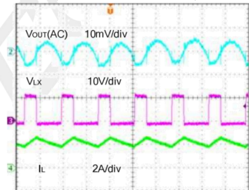
Output Ripple
