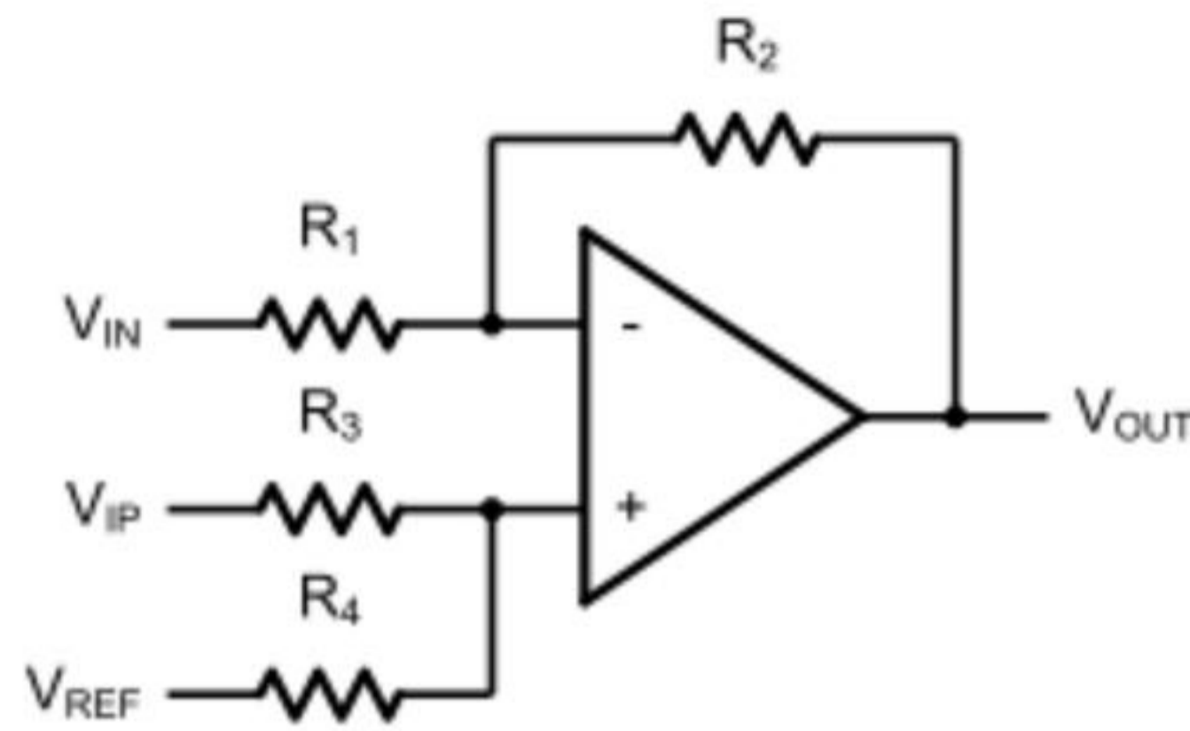
Figure 4. Differential Amplifier
