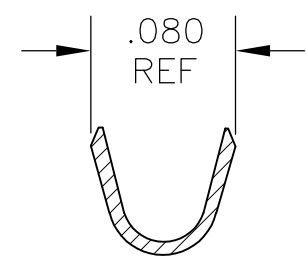
INSULATION RANGE .061 MAX SECTION A-A
