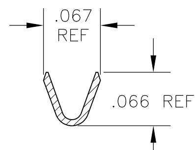
WIRE RANGE #22-#26 SECTION B-B
