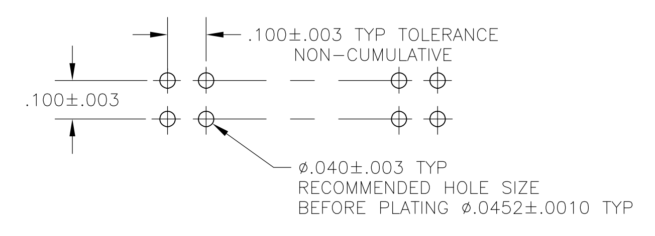
RECOMMENDED HOLE LAYOUT
