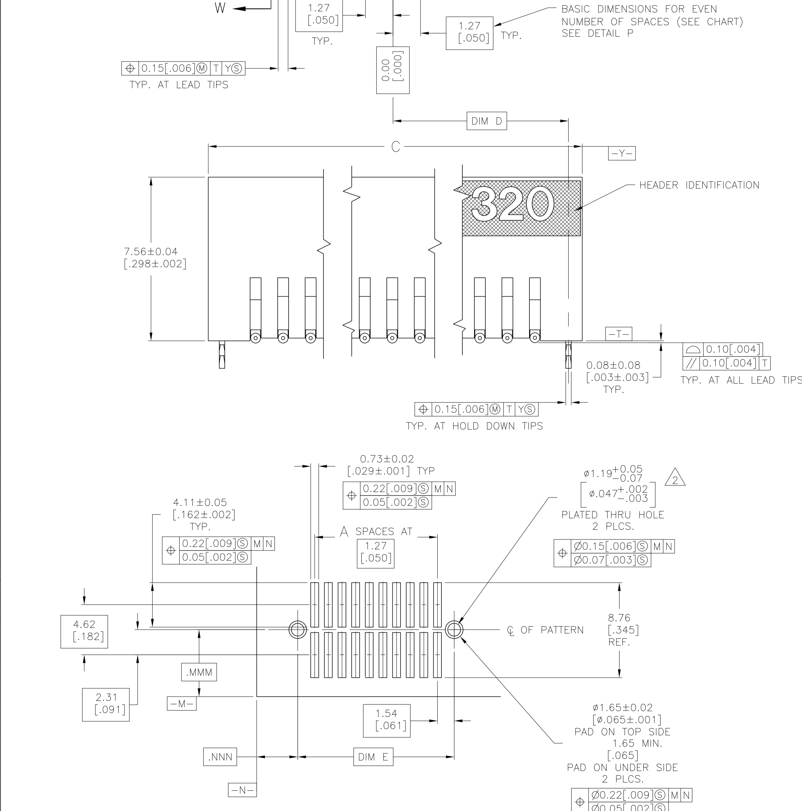
RECOMMENDED BOARD LAYOUT SCALE 5:1
