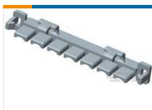
TE Part #1-1969609-1 11P VAL-U-LOK TPA 26-22 AWG
