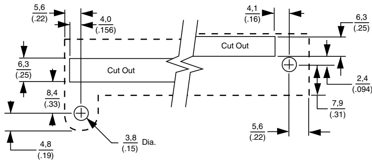
Right Angle Mounting Panel Layout
