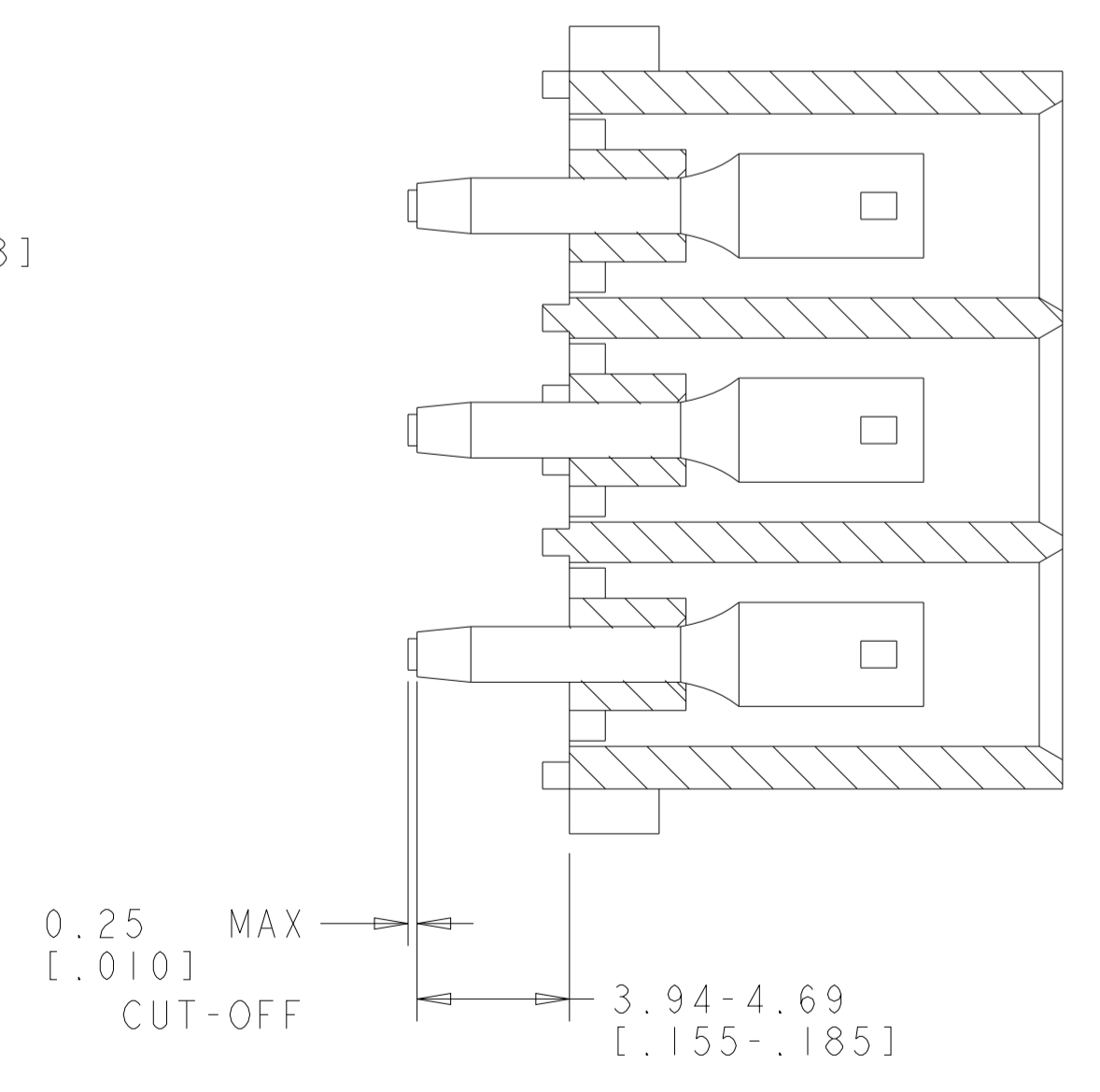
SECTION B-B
