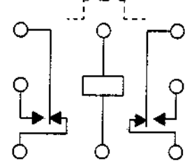
TERMINAL VIEW
