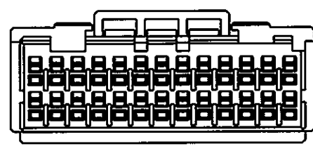
26POS(X-KEY): 1-1827863-3
