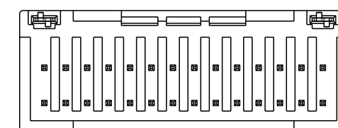
28POS(X-KEY) 1-1871315-4
