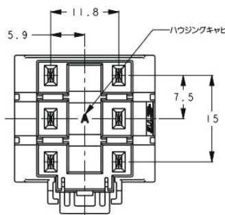
Receptacle Assembly
