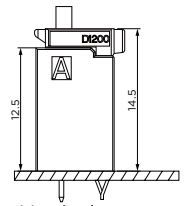
Vertical type
