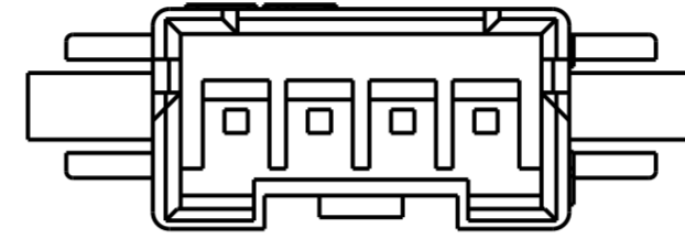
4 POSITION 1969590-4
