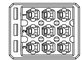
9POS(X-KEY): 1-2040444-3
