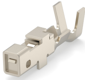
Receptacle Contact (for Receptacle housing)
