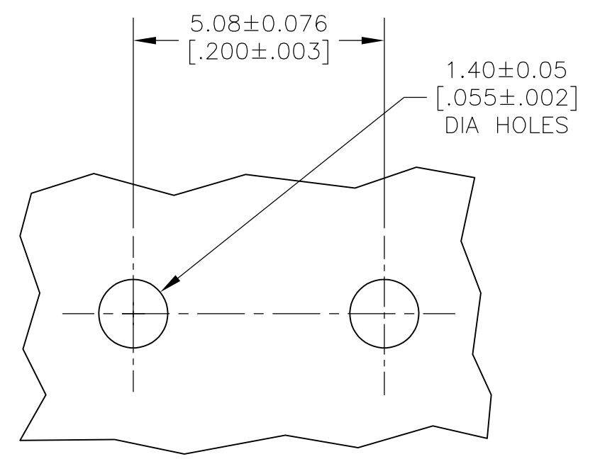
P.C. BOARD HOLES
