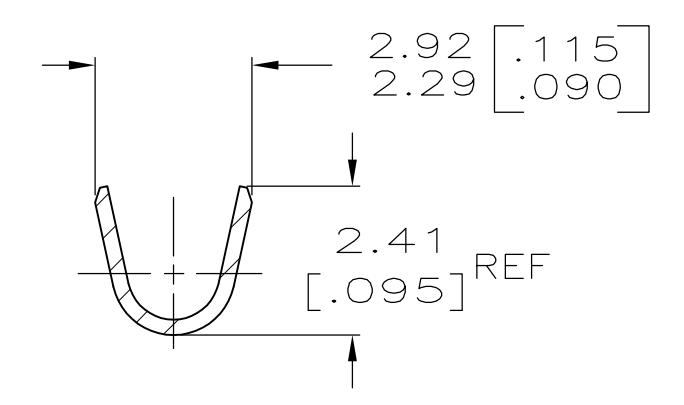
SECTION C-C SCALE 8:1
