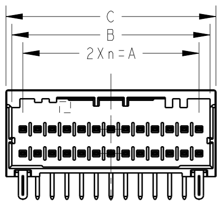
26POS(X-KEY): 1-2271888-3
