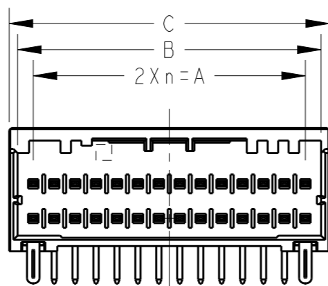
28POS(X-KEY): 1-2271888-4
