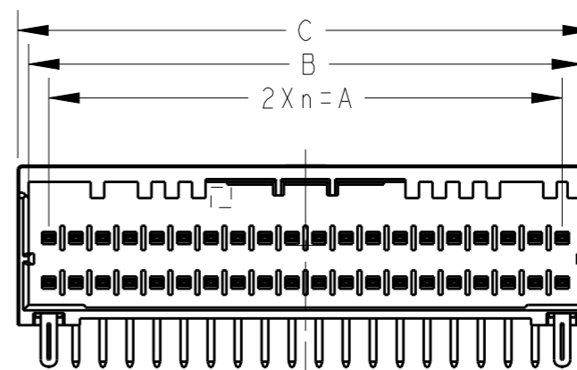
40POS(X-KEY): 1-2271888-0
