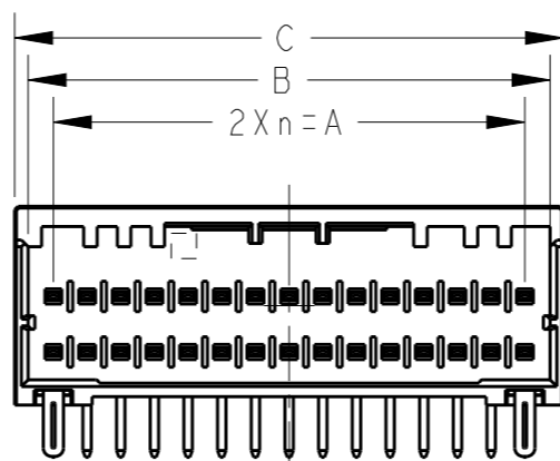
30POS(X-KEY): 1-2271888-5
