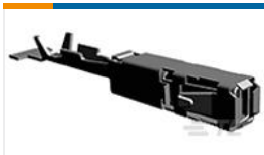
TE Part #1418884-1 AMP MCP 1.5K, CONTACT, SWS
