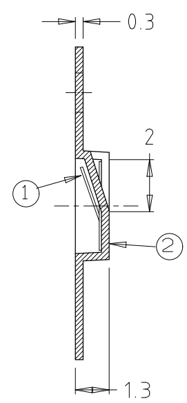
SECT. A-A
