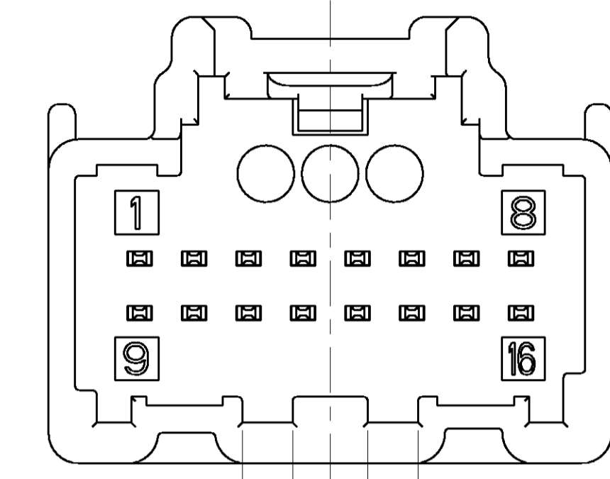
(1.75) (1.75) (4.10) (4.10) KEY CODE "E" SCALE 4:1
