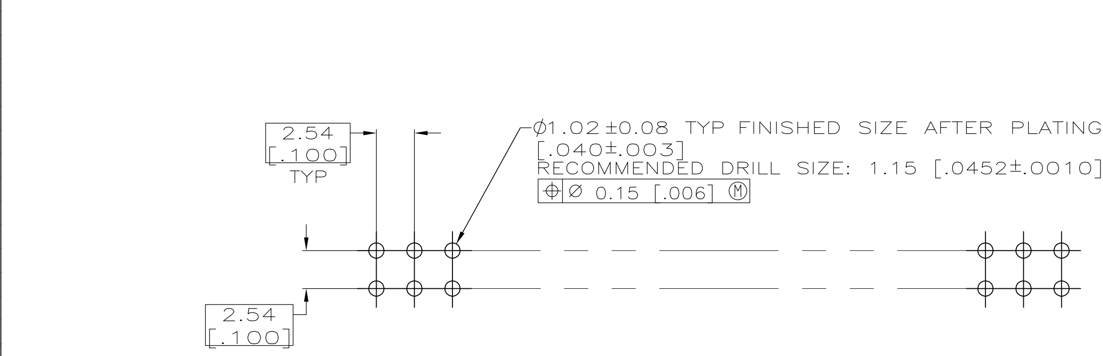
RECOMMENDED MOUNTING HOLE LAYOUT
