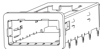
Behind-Bezel Cage
