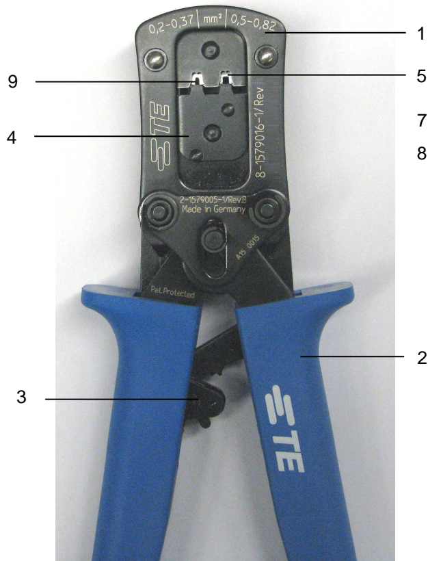
Picture 1: Hand tool components
