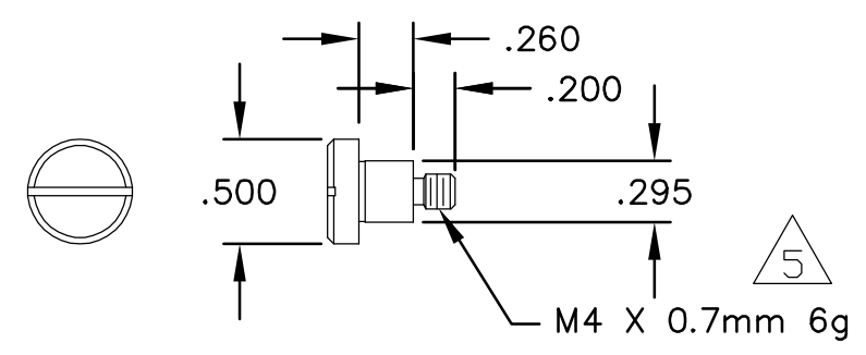
SHOULDER SCREW (REFERENCE ONLY)
