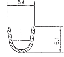
SECT. B-B
